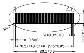
DETAIL A(2.5:1)
